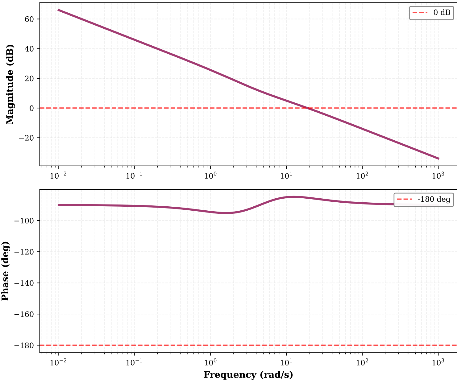
Bode Diagram of Loop Transfer Function C(s)G(s)
