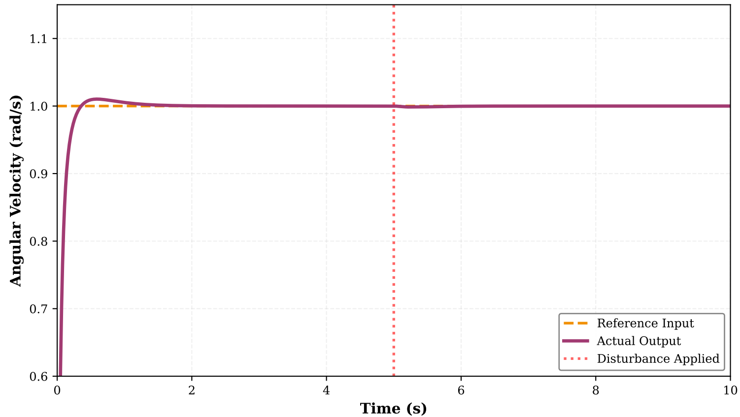
Disturbance Rejection (20% Load Disturbance at t=5s)
