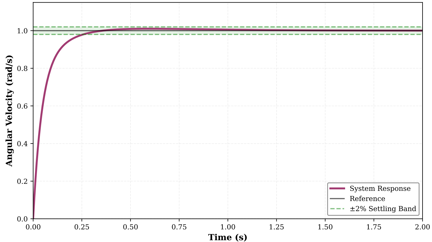
Closed-Loop Step Response with Settling Characteristics
