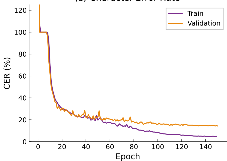
(b) Character Error Rate
