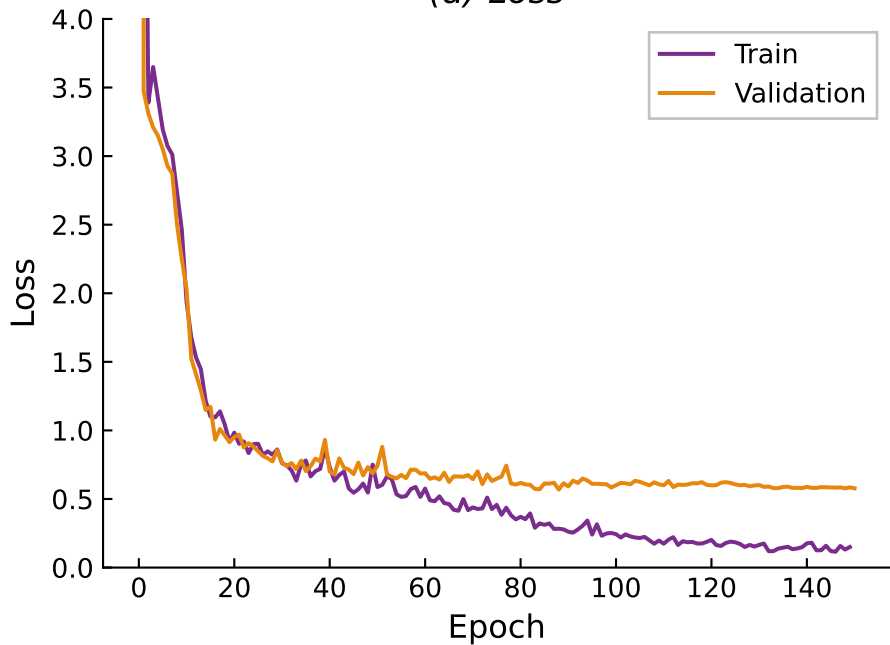
(a) Loss
