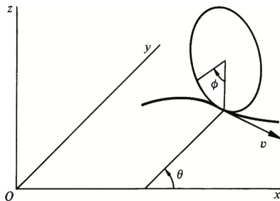
Figure 1: Vertical disc rolling on a horizontal plane
