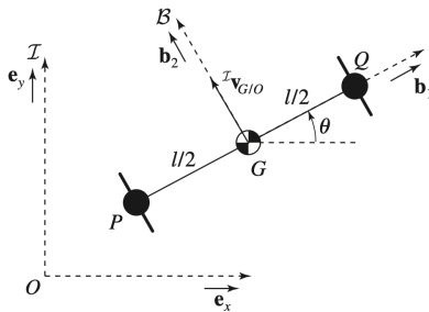
Figure 2: Simple nonholonomic system. The particles P and Q are constrained to move along the directions of the blades
