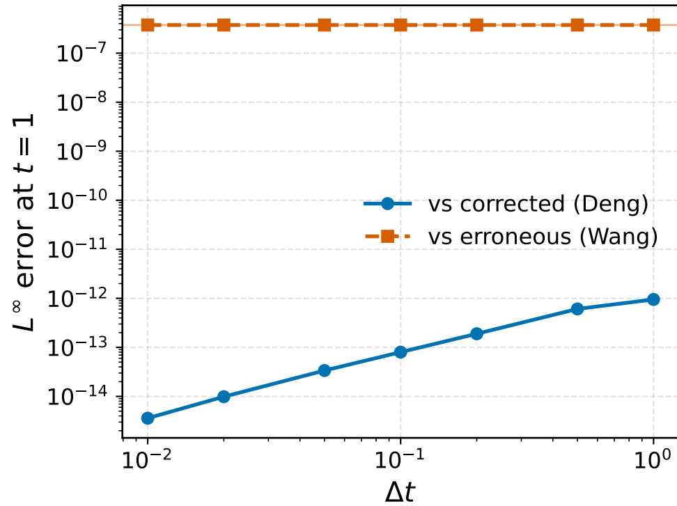
Temporal refinement ( N = 20 )
