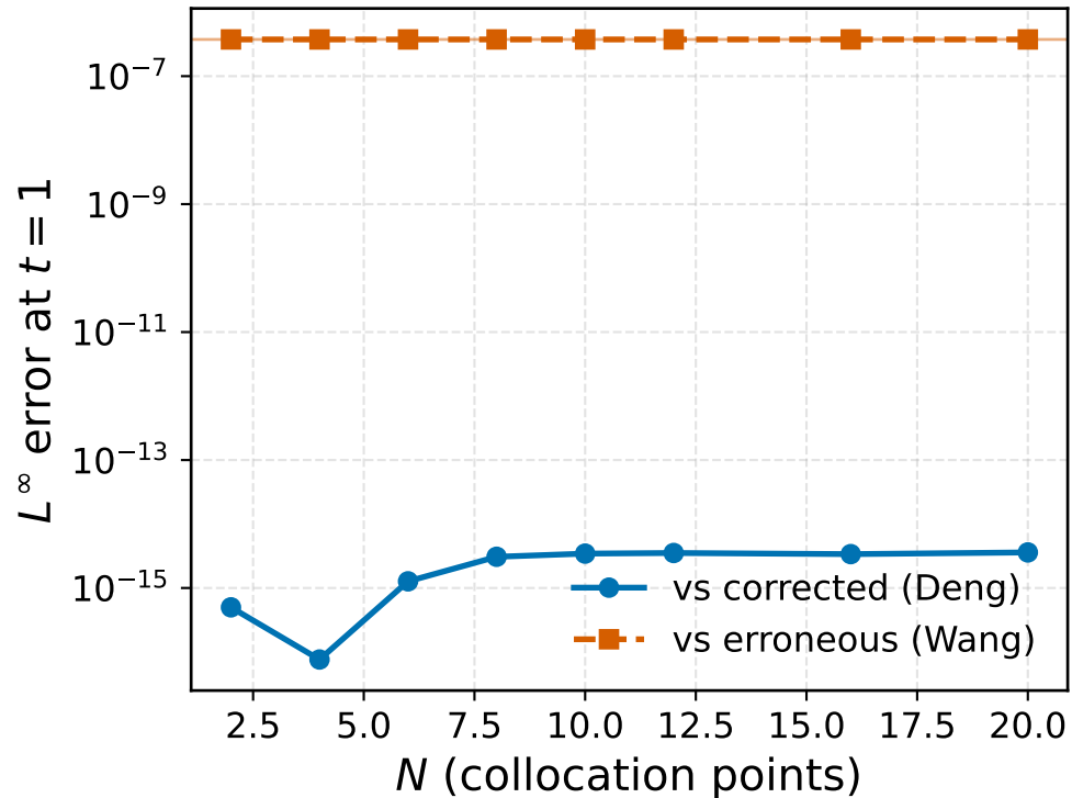
Spatial refinement ( \Delta t = 10^{-2} )
