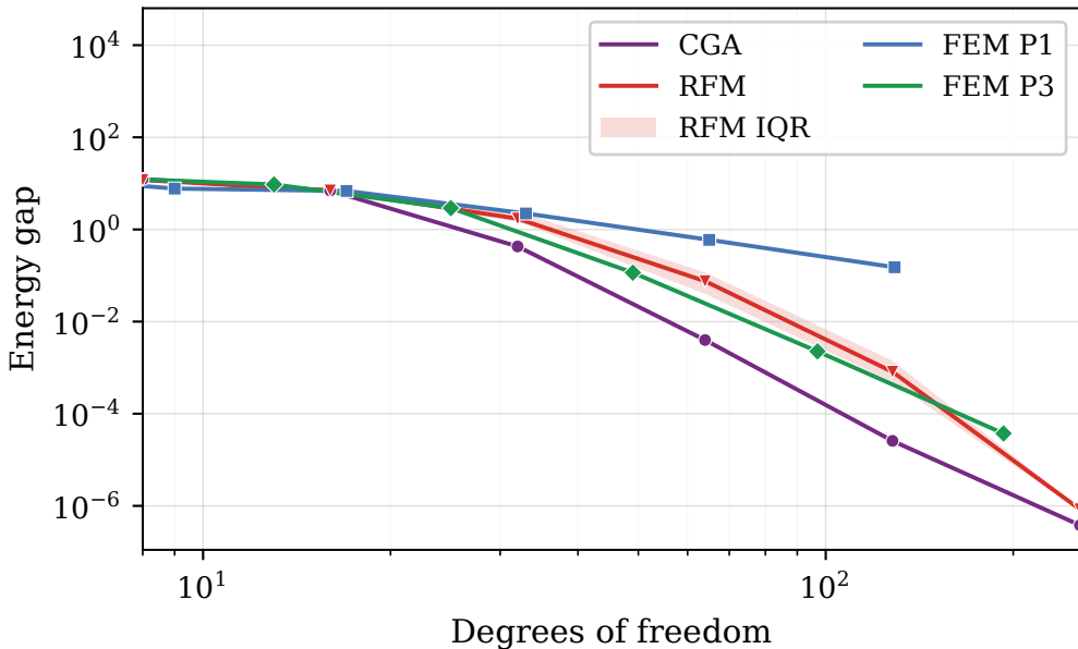
Linear, d=1
