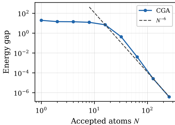
Cubic semilinear problem, d=1
