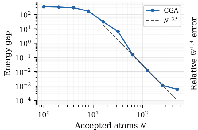
Reaction p=4 problem, d=2, k=3
