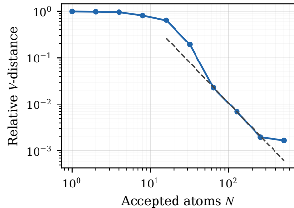
Reaction p=4 problem, d=2, k=3
