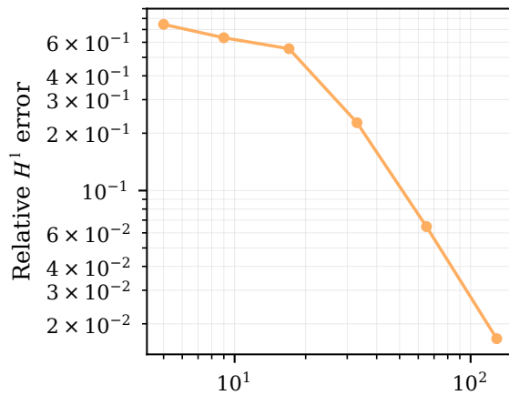
Cubic, d=1
