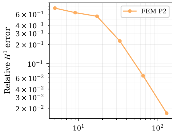
Linear, d=1
