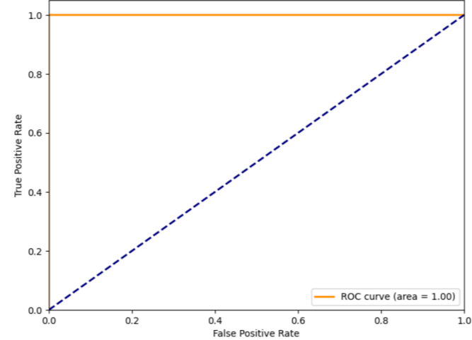
Receiver Operating Characteristic for SSL Renegotiation with frac=1.0 and n_estimators=100
