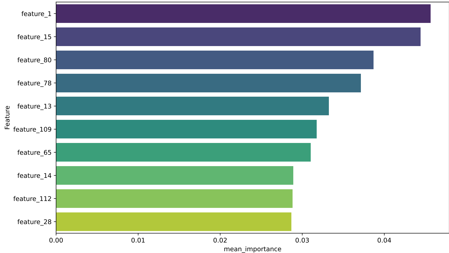
Top 10 Features by Mean Importance
