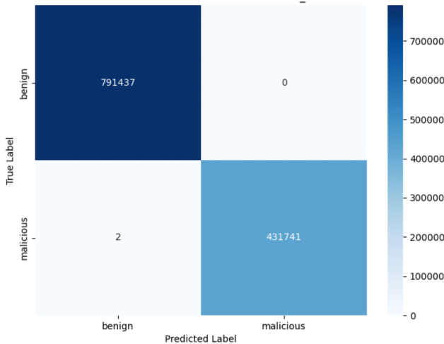
Confusion Matrix for SSDP Flood with frac=1.0 and n_estimators=100
