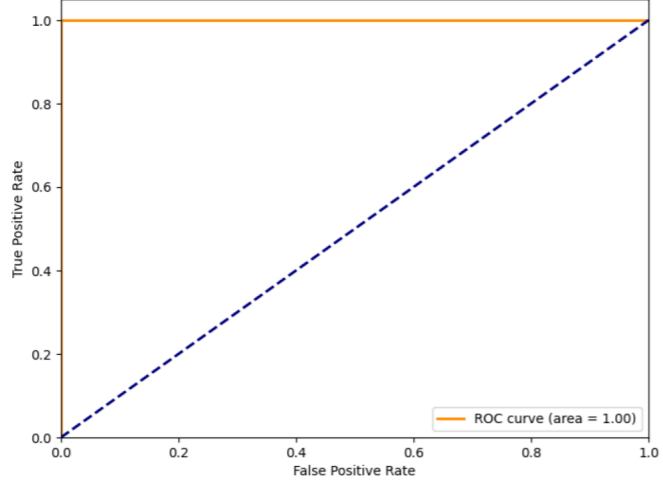
Receiver Operating Characteristic for OS Scan with frac=1.0 and n_estimators=100
