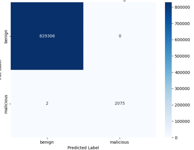
Confusion Matrix for SYN DoS with frac=1.0 and n_estimators=100
