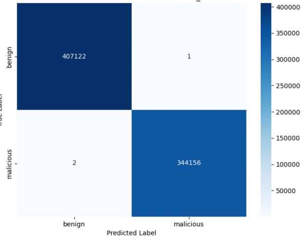
Confusion Matrix for ARP MitM with frac=1.0 and n_estimators=100
