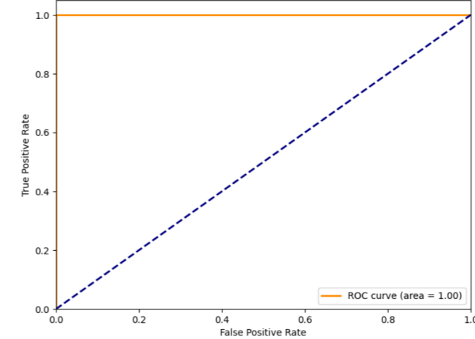
Receiver Operating Characteristic for Mirai Botnet with frac=1.0 and n_estimators=100
