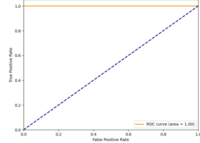
Receiver Operating Characteristic for ARP MitM with frac=1.0 and n_estimators=100
