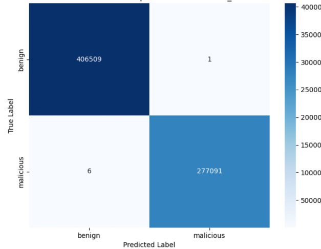
Confusion Matrix for Active Wiretap with frac=1.0 and n_estimators=100
