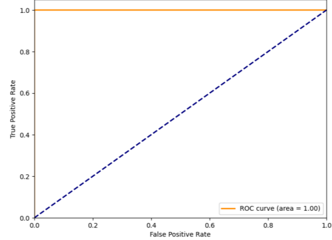
Receiver Operating Characteristic for Fuzzing with frac=1.0 and n_estimators=100
