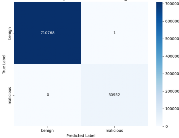
Confusion Matrix for Video Injection with frac=1.0 and n_estimators=100
