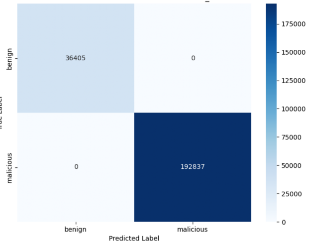
Confusion Matrix for Mirai Botnet with frac=1.0 and n_estimators=100
