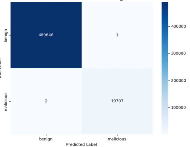
Confusion Matrix for OS Scan with frac=1.0 and n_estimators=100
