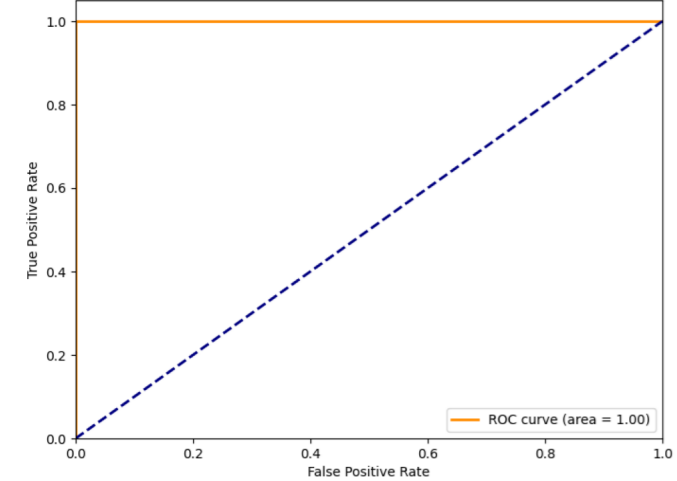
Receiver Operating Characteristic for SSDP Flood with frac=1.0 and n_estimators=100
