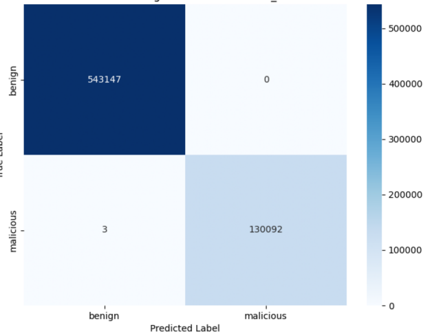
Confusion Matrix for Fuzzing with frac=1.0 and n_estimators=100
