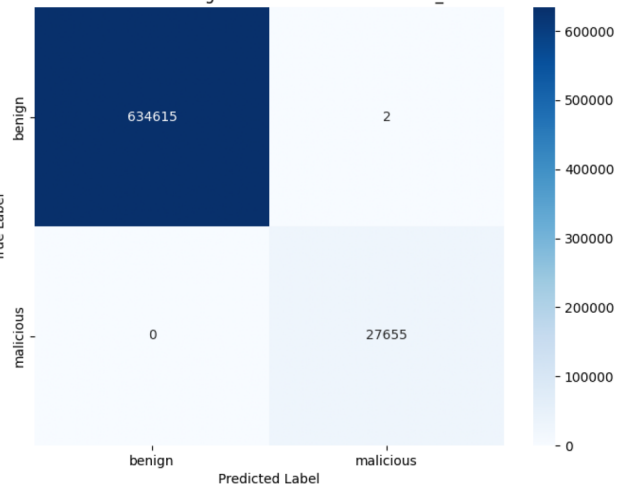
Confusion Matrix for SSL Renegotiation with frac=1.0 and n_estimators=100
