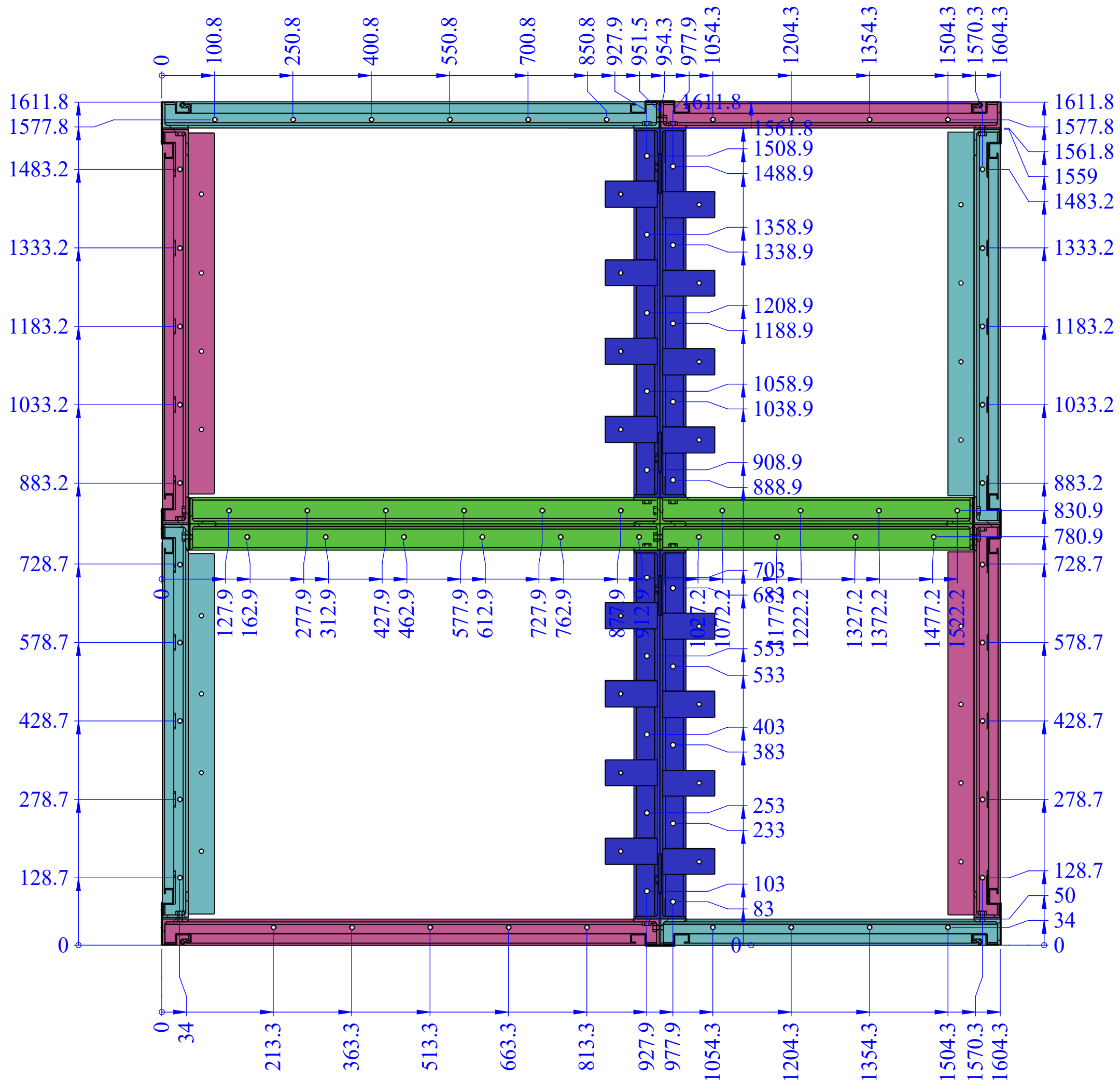
BOTTOM HOLES OF MIDDLE FRAME FOR FIXING BASE FRAME
