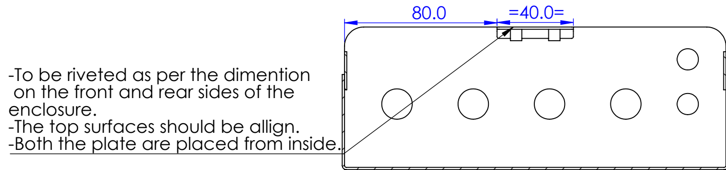
SECTION C-C
