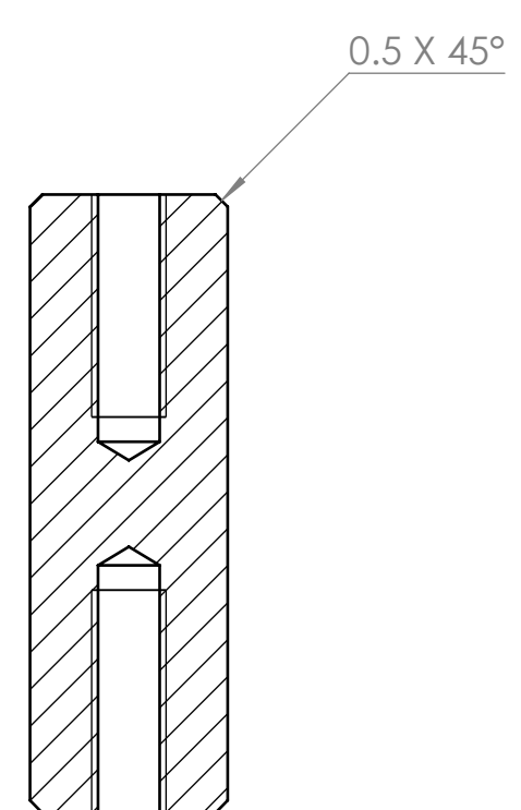
SECTION K-K SCALE 3 : 1
