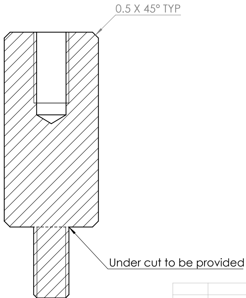
SECTION K-K
