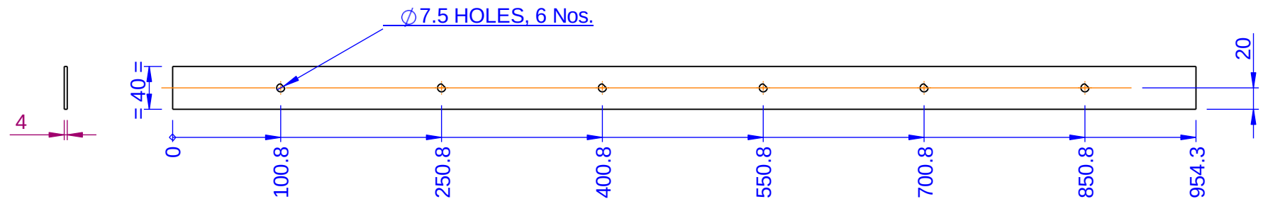
GASKET 1- BASE FRAME (QTY : 1 No.) MATERIAL : GIVEN
