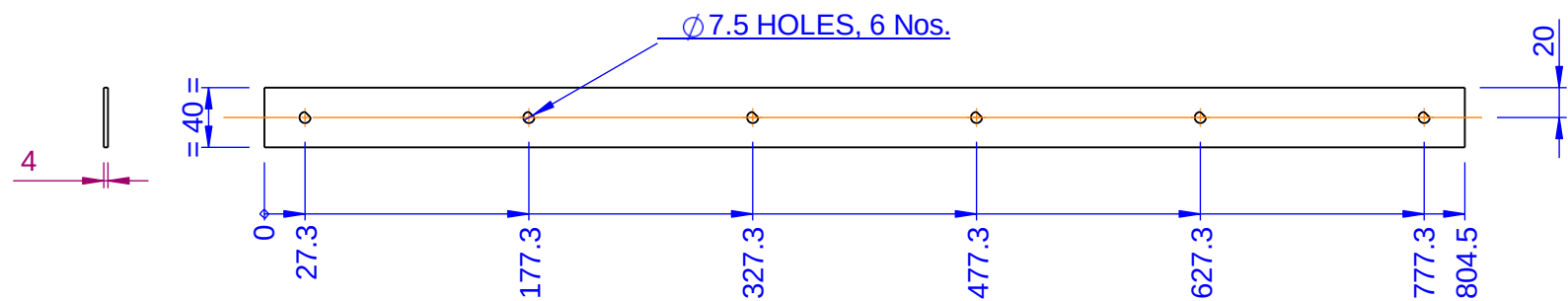
GASKET 2 - BASE FRAME (QTY : 1 No.) MATERIAL : GIVEN
