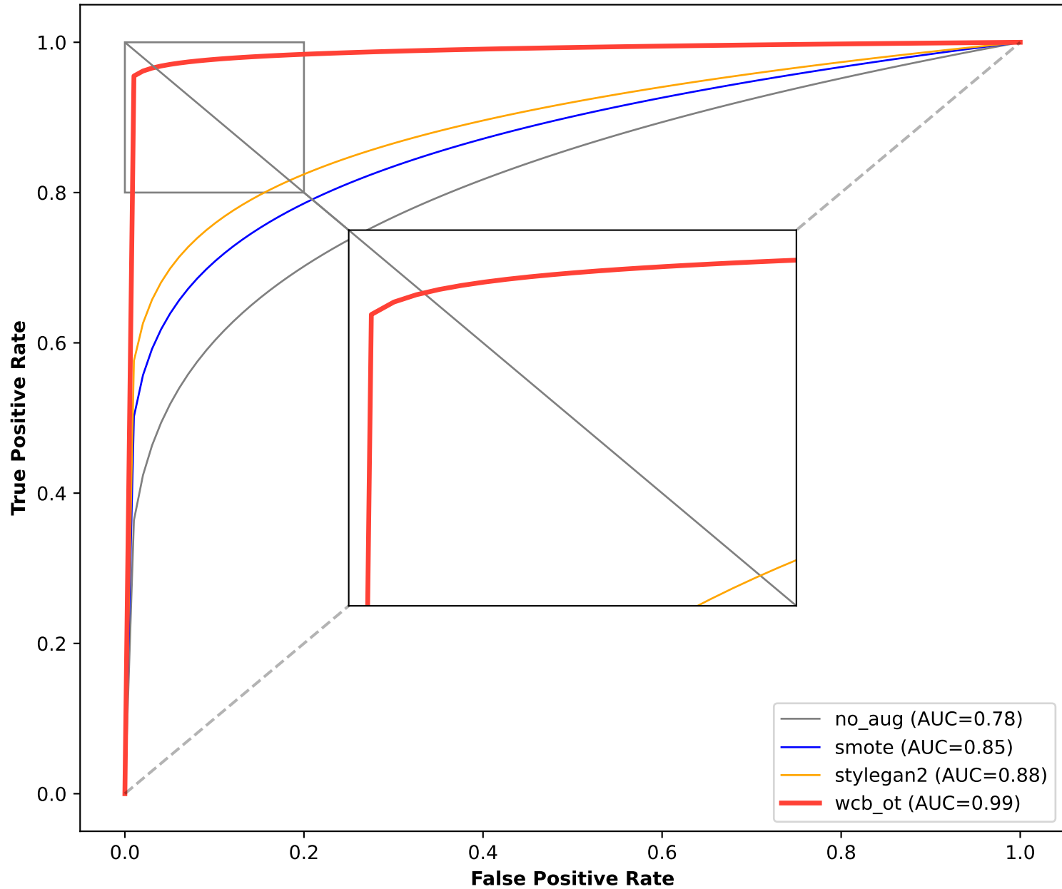
Figure 12: ROC Curves — Rare Malignancy Detection
