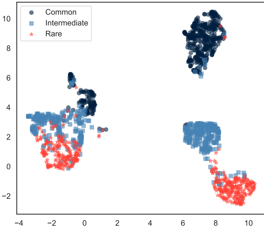
UMAP Visualization of Feature Space
