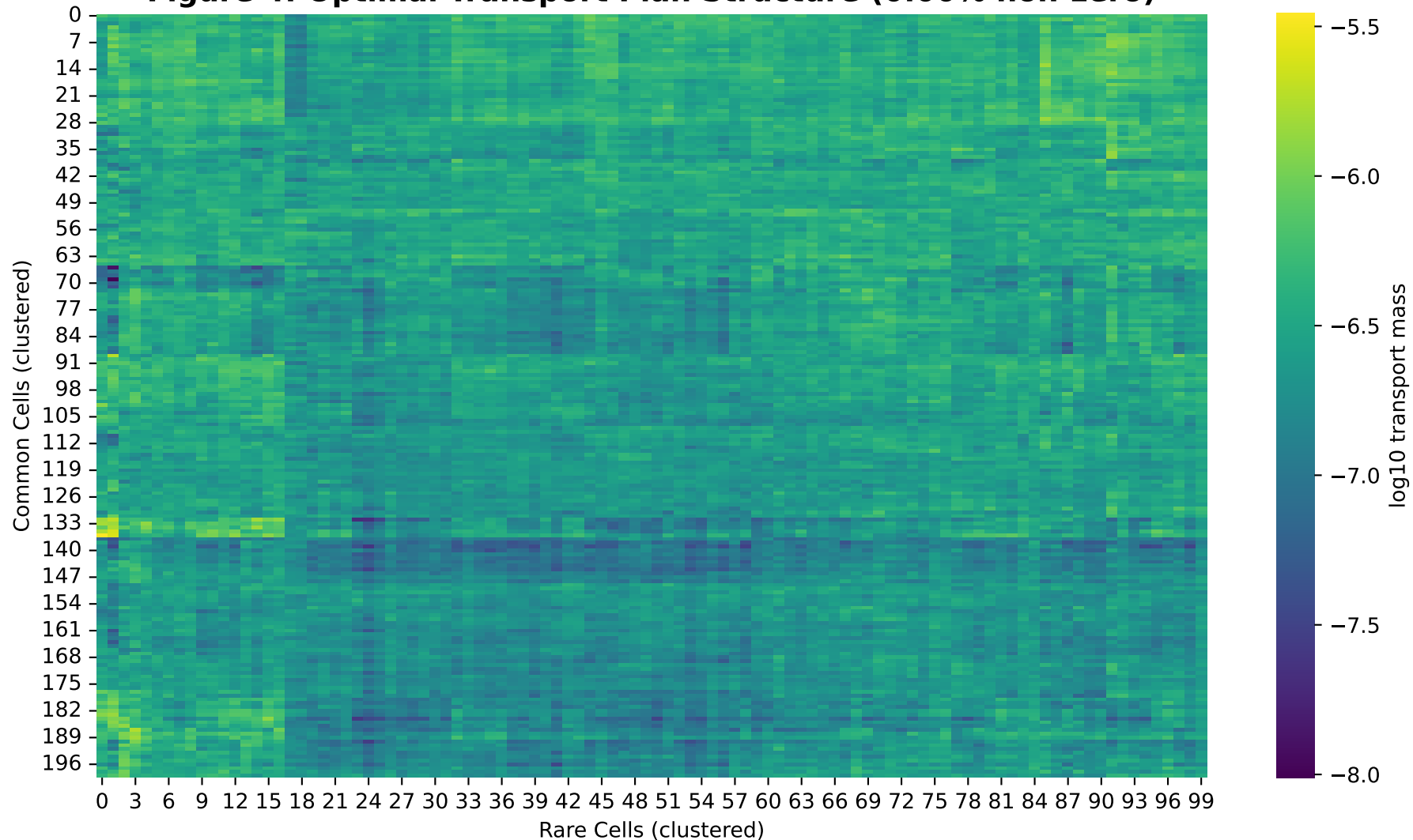
Figure 4: Optimal Transport Plan Structure (0.00% non-zero)
