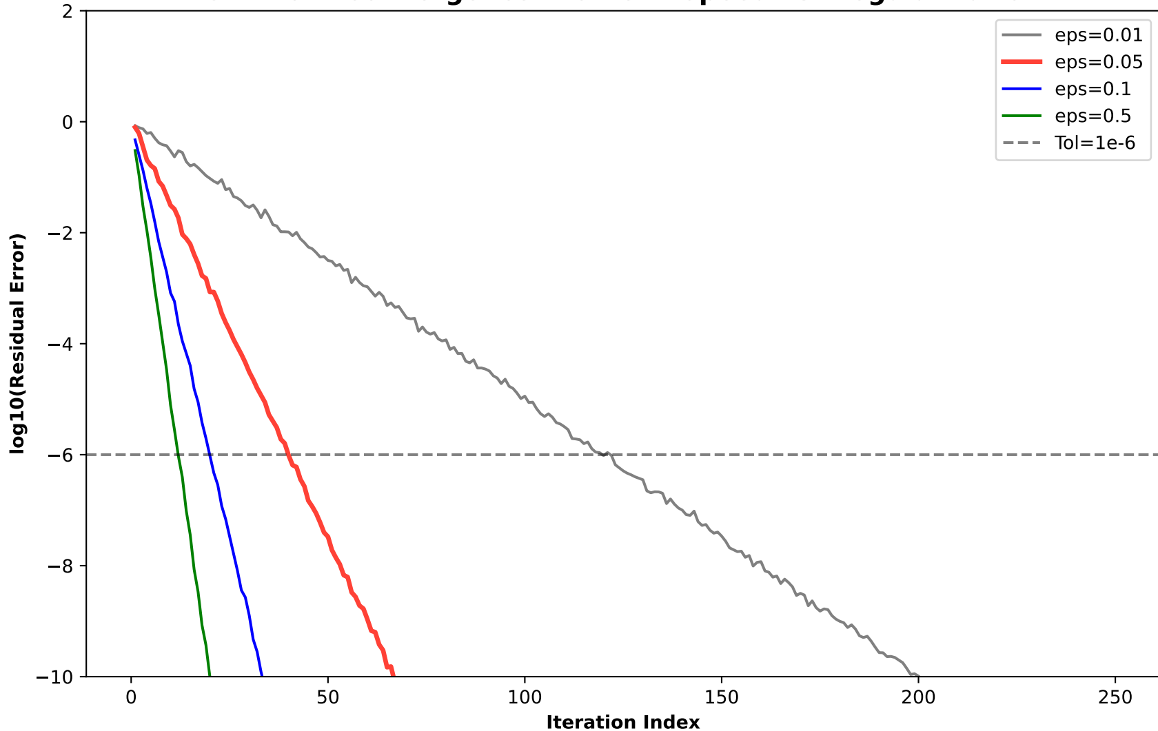
Sinkhorn Convergence Profile — Speed vs. Regularization
