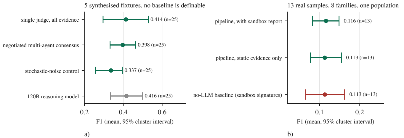
Figure 1: Every measured arm on one F1 axis. a) the synthesised fixtures, b) the real-sample population.
