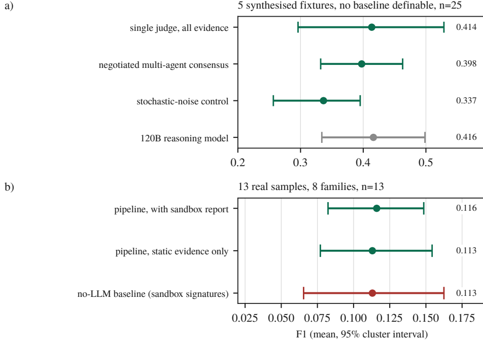
Figure 2: Every measured arm on one F1 axis. a) the synthesised fixtures, b) the real-sample population. Points are means over per-sample F1, bars are 95% intervals resampling the cluster the observations are independent at.
