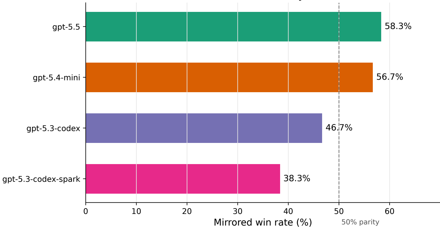
Mirrored Win Rate By Model
