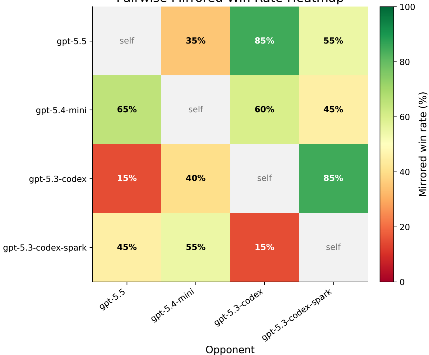
Pairwise Mirrored Win Rate Heatmap
