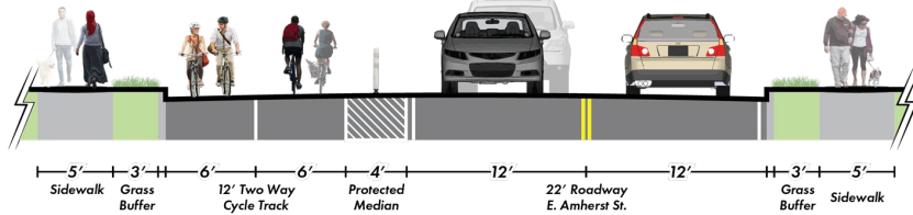
East Amherst St Proposed Conditions
