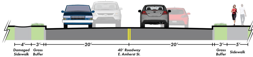
East Amherst St Existing Conditions
