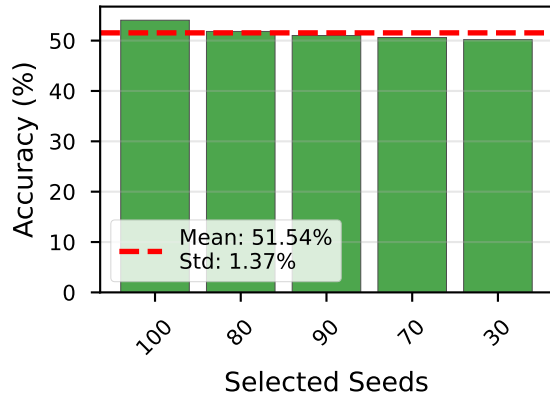
Best 5 Seeds
