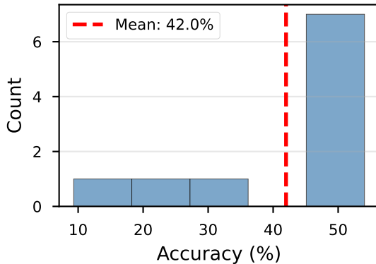
Accuracy Distribution
