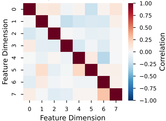
Standard Barlow Twins ( \tau=1.0 , View-Invariance)
