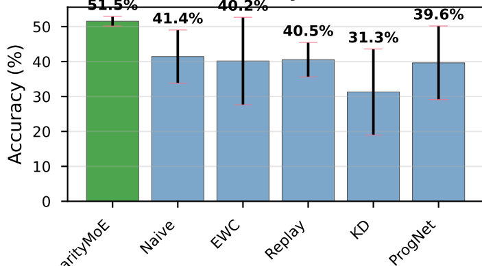
Final Accuracy (5 seeds)
