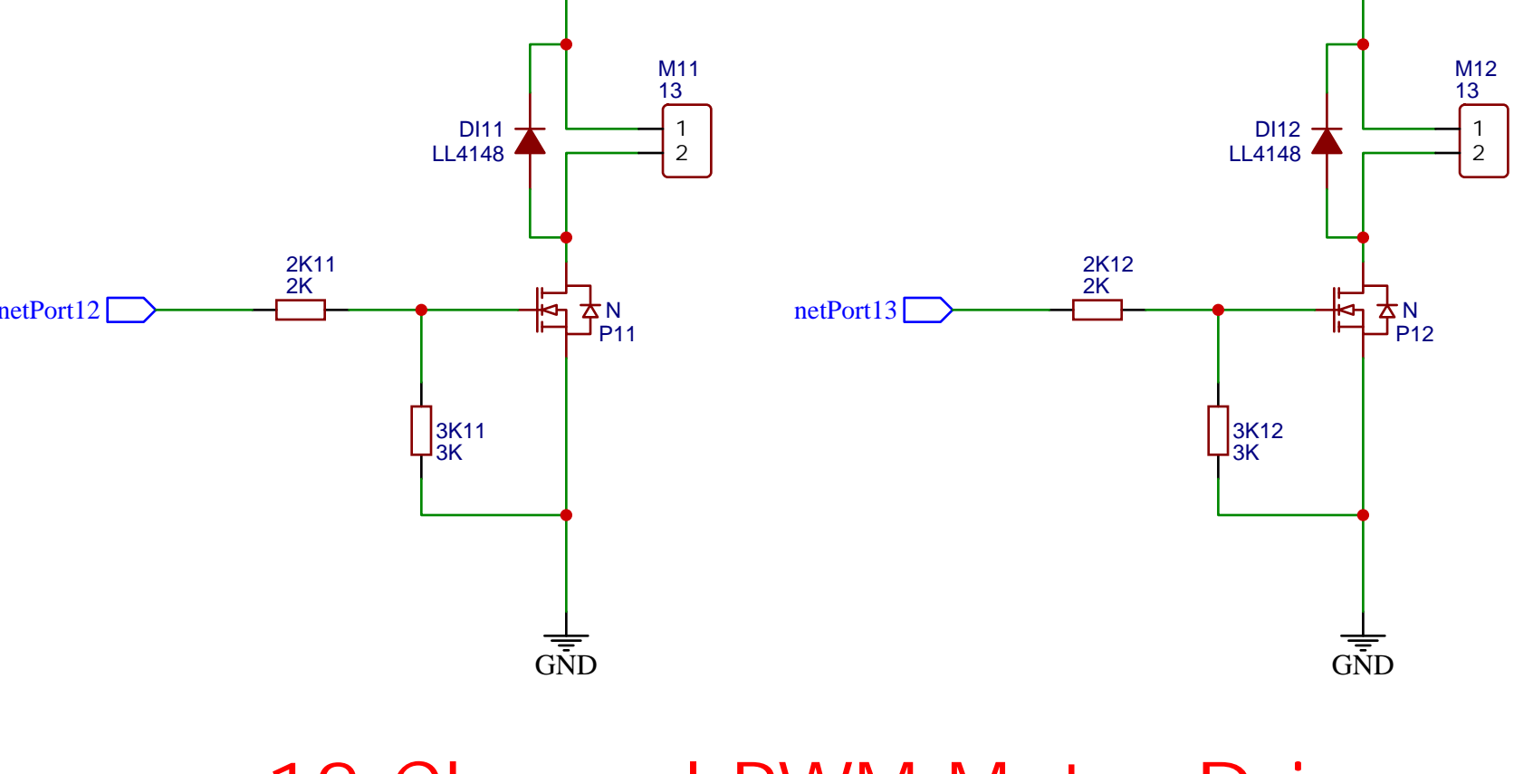
12 Channel PWM Motor Driver
