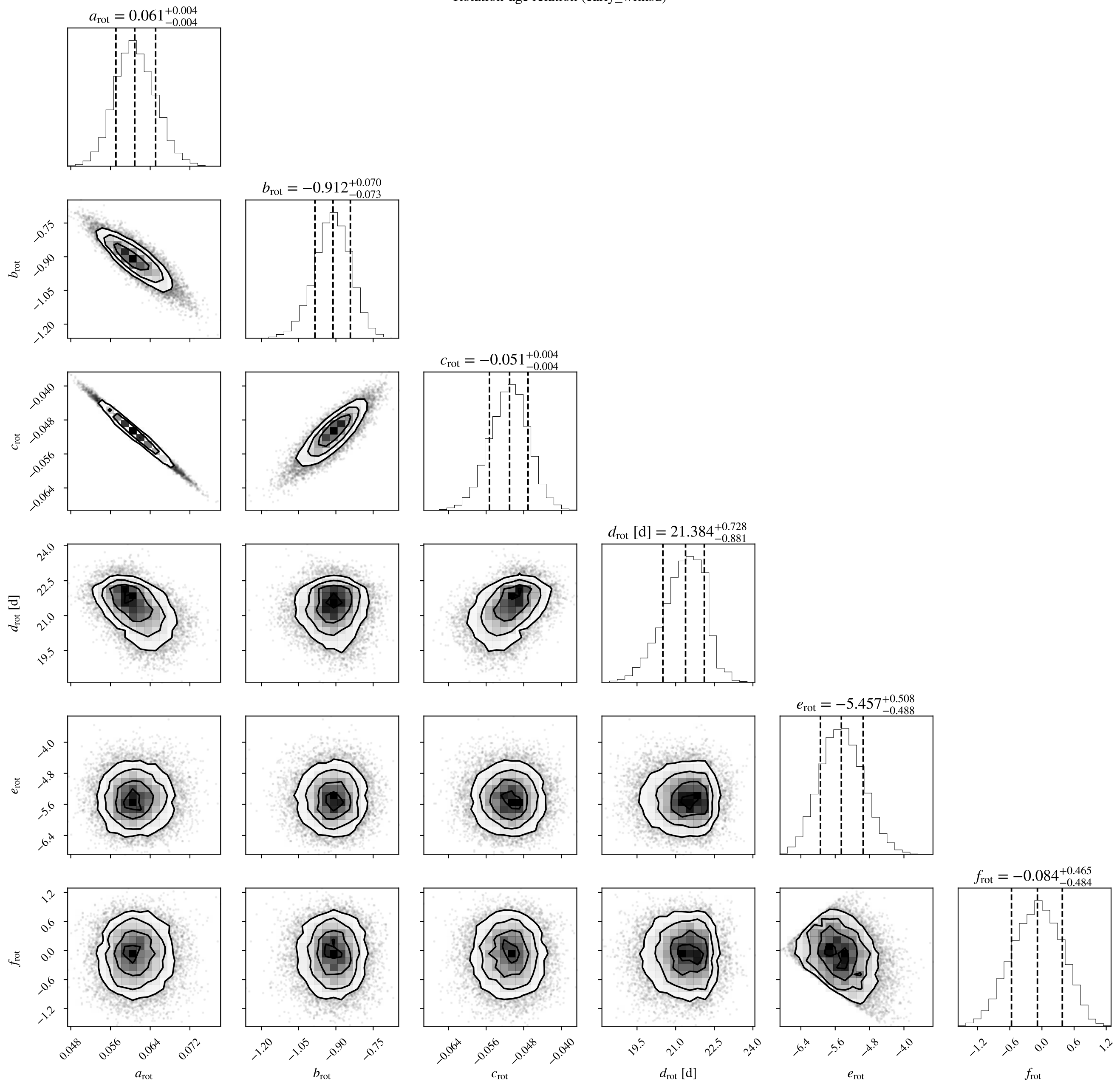
Rotation-age relation (early_withsd)
