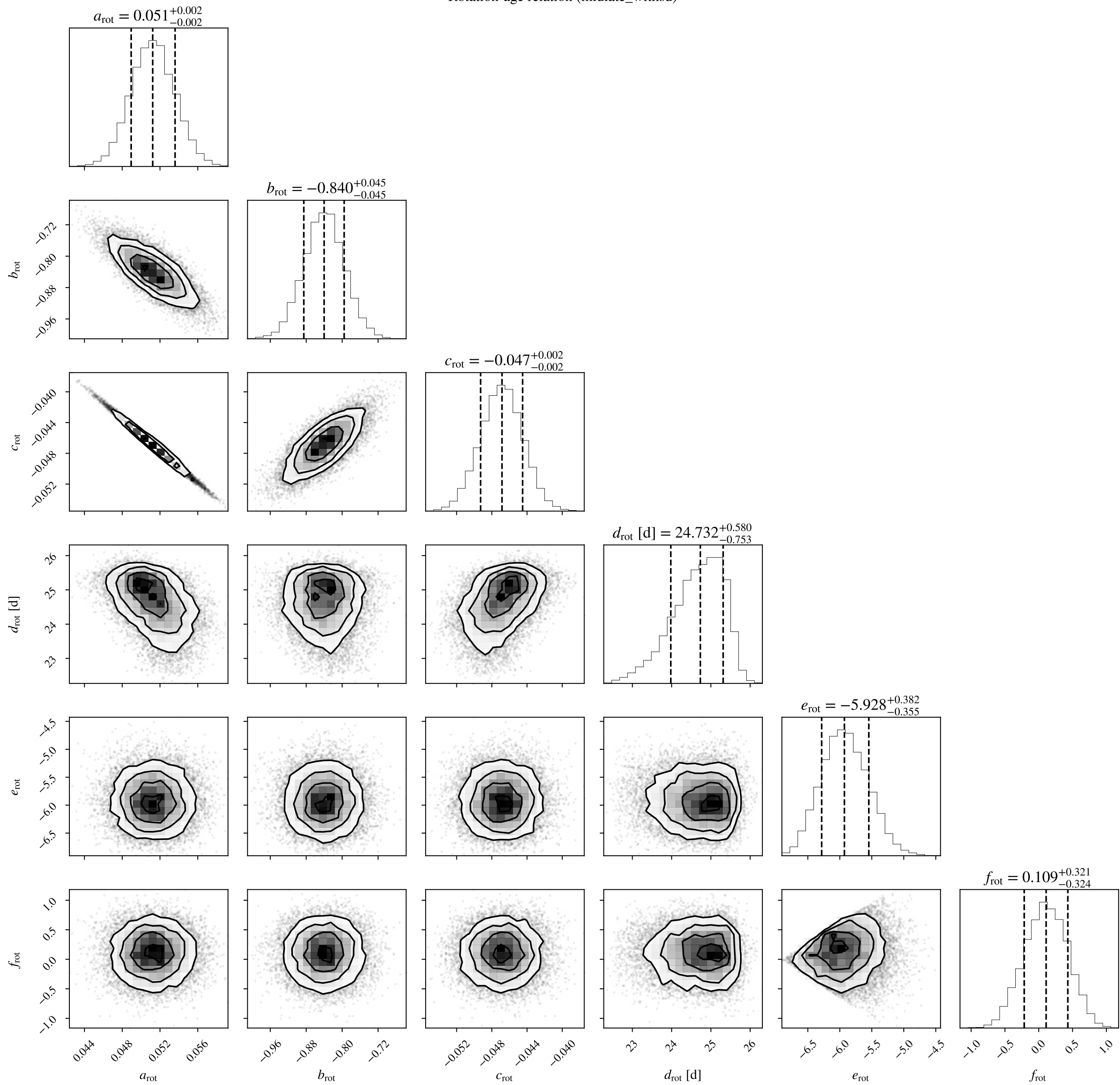
Rotation-age relation (midlate_withsd)
