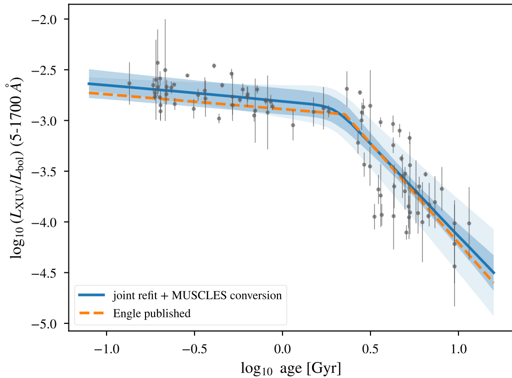
Engle relations: published vs joint refit (midlate_withsd)
