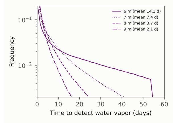
This model
