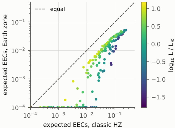
Per star (each zone's own survey)
