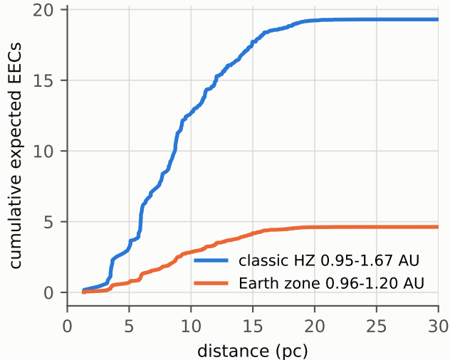
Where the yield comes from
