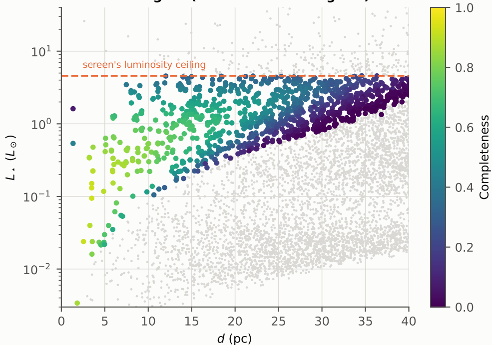
Selected targets (cf. Stark+2024 Fig. 11)
