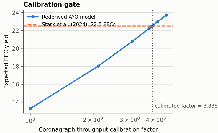
Figure 1: Modelled yield against the coronagraph throughput calibration factor, with the published 22.5-candidate target.
