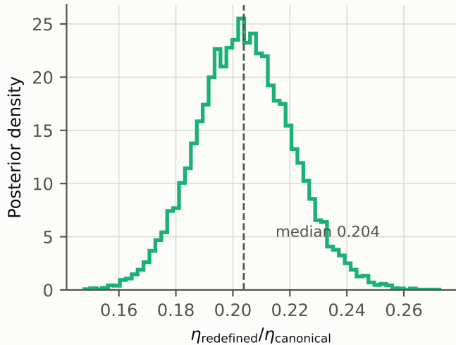
Ratio: \Gamma cancels exactly
