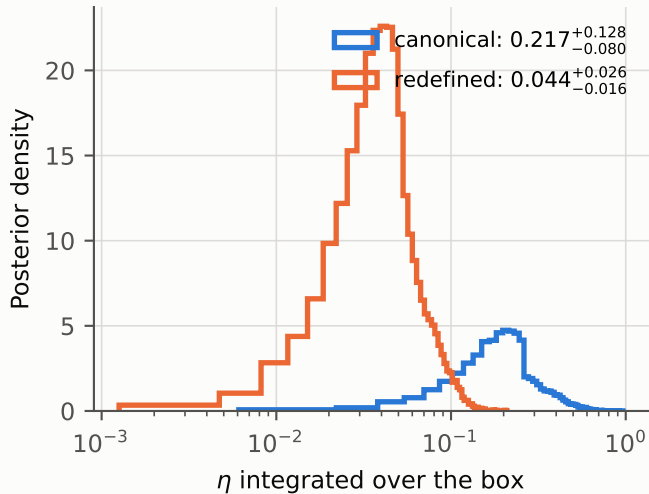
Occurrence rate per box
