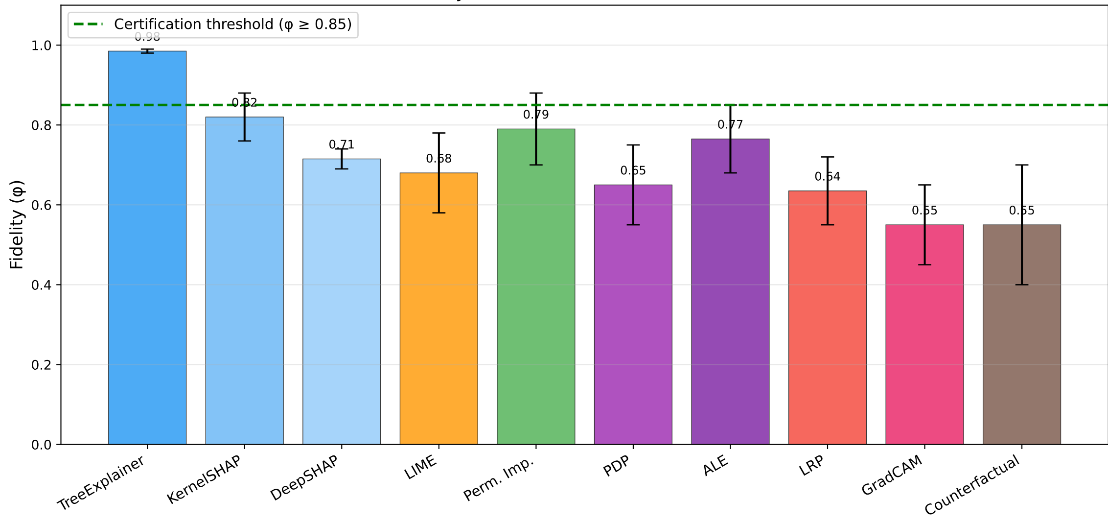
Fidelity Scores Across Post-Hoc Methods
