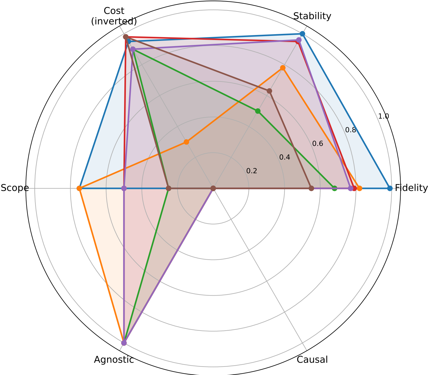
Six-Axis Radar Comparison of Post-Hoc Explanation Methods
