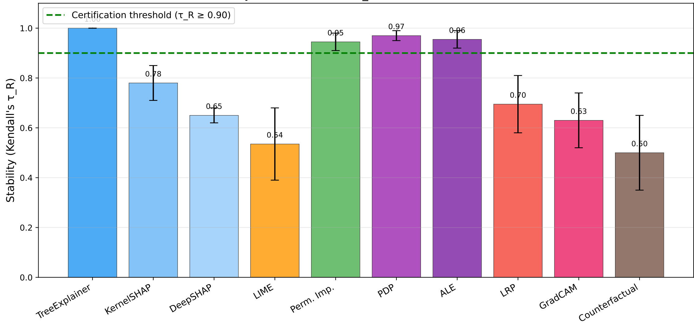
Stability Scores (Kendall's \tau_R ) Across Post-Hoc Methods
