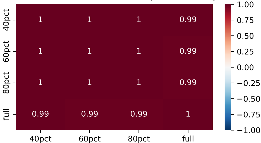
HMM Parameter Correlations (vs Full Model)
