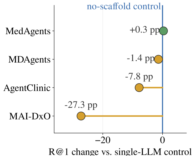
Figure 5: Effect of multi-agent scaffolding, measured as each scaffold’s variant-aware R@1 change (percentage points) relative to the no-scaffold single-LLM control on Phenopacket-Store with the Gemini Flash backbone. The vertical line at zero is the control; a marker to its right (green) beats the control and to its left (gold) trails it. Only MedAgents essentially matches the control (+0.3 pp); MDAgents (−1.4 pp), AgentClinic (−7.8 pp), and MAI-DxO (−27.3 pp) all fall below it. Deepening the scaffold therefore does not reliably improve over a single well-prompted LLM call on this task.
