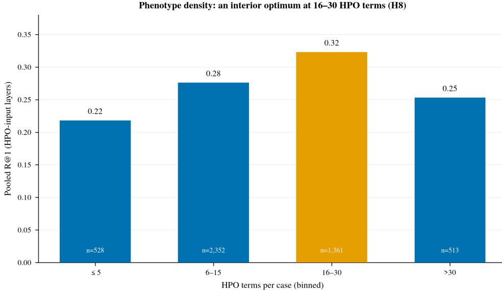
Figure 5: Phenotype-density inverted-U (H8) . Pooled R@1 on the HPO-input layers peaks at 16–30 HPO terms per case; both under- and over-specified inputs degrade accuracy.
