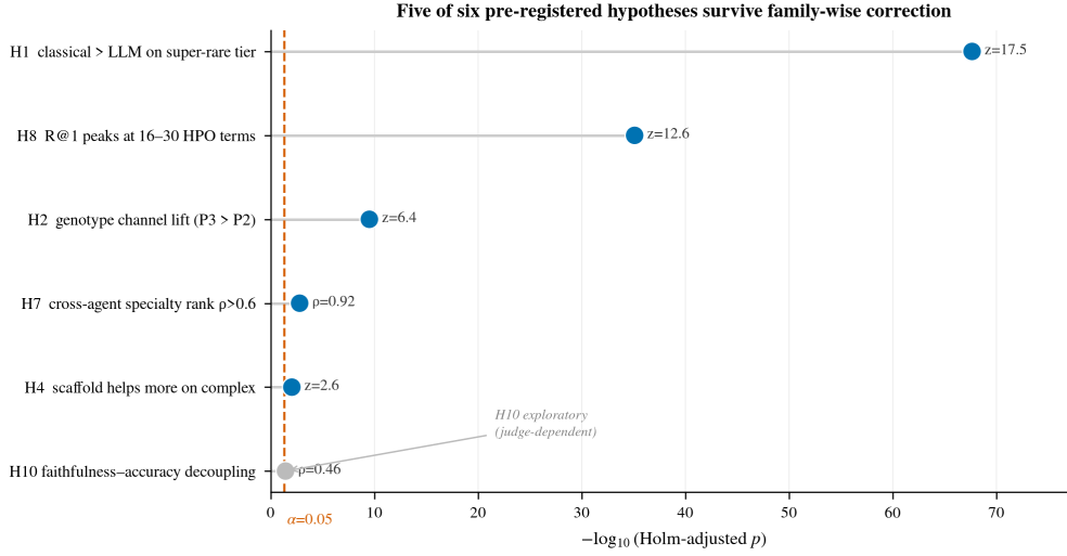
Figure 6: Pre-registered hypothesis tests. Forest plot of -\log_{10}(\text{Holm-adjusted } p) for the six testable hypotheses; five survive family-wise correction at \alpha=0.05 . H10 (faithfulness-accuracy decoupling) is reported as exploratory and judge-dependent.
