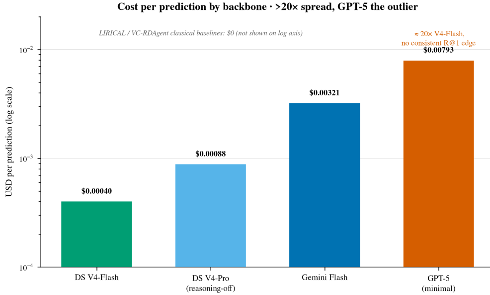
Figure 12: Cost per prediction by backbone (log axis); >20× spread, classical baselines at $0.
