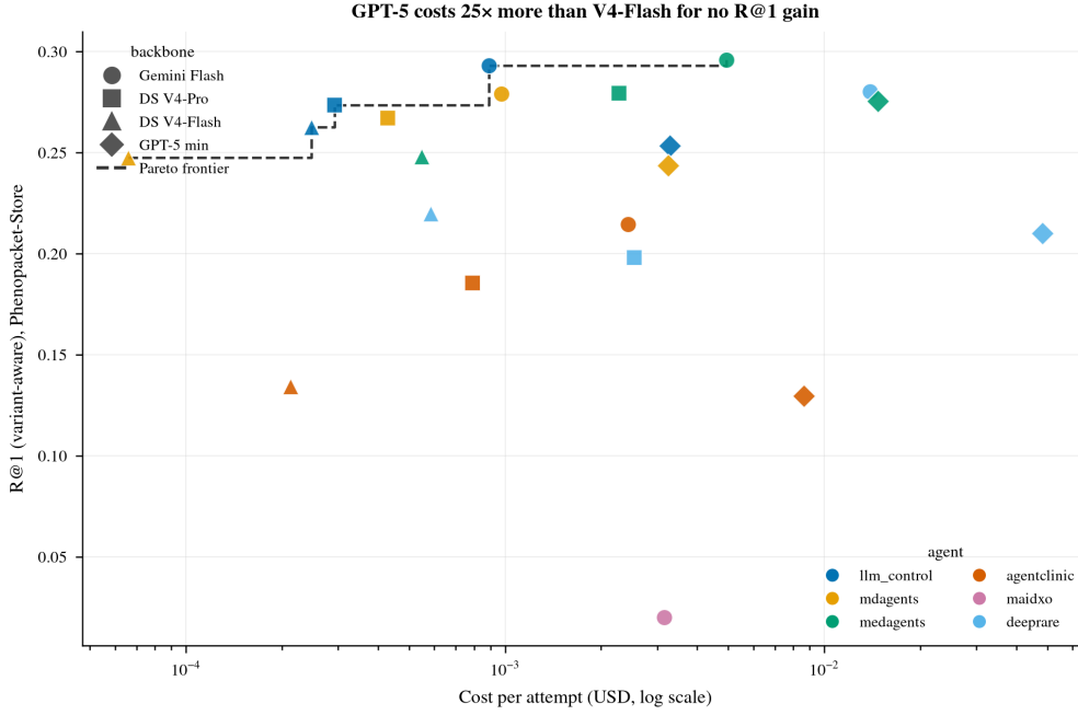
Figure 3: Cost vs. accuracy (F3/F4) . Each marker is one agent \times backbone cell on Phenopacket-Store (log cost-per-attempt axis, attempted denominator); dashed line is the Pareto frontier. GPT-5 minimal (diamonds) sits far right at \sim 25\times the cost of DeepSeek V4-Flash with no R@1 gain.
