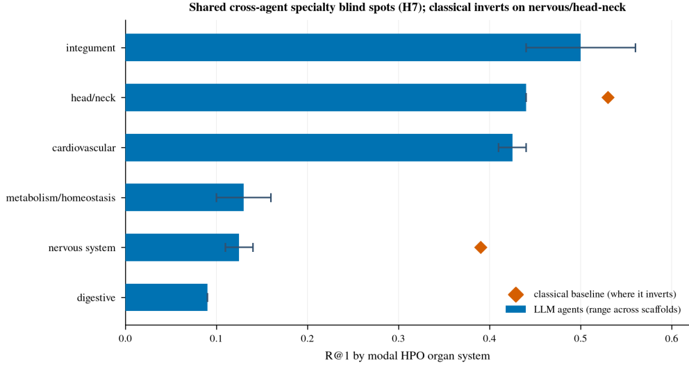
Figure 11: H7 cross-agent per-specialty R@1 (modal HPO organ-system axis). Bars span the R@1 range across LLM scaffolds; the shared weak specialties (digestive, metabolic, nervous) indicate ontology/data-level difficulty rather than agent-specific blind spots. Diamonds mark where the classical baselines invert the LLM weakness (nervous, head/neck).
