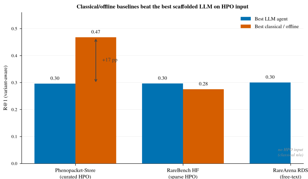
Figure 2: Classical/offline baselines beat the best scaffolded LLM on HPO input (F1). Best variant-aware R@1 per data layer, LLM agents vs. classical/offline baselines (attempted denominator, common N=2000 on PP-Store/RareArena). On curated HPO (Phenopacket-Store) LIRICAL leads the best LLM by 17 pp; on free-text RareArena no classical baseline runs (no HPO input).
