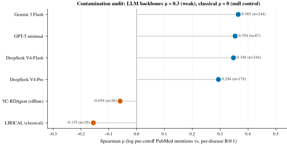
Figure 10: A6 TS-Guessing contamination audit. Spearman \rho between log pre-cutoff PubMed mentions and per-disease R@1, per backbone. Every LLM backbone clusters at \rho \approx 0.3 (weak positive); both classical/offline baselines sit at \rho \approx 0 (null control), confirming the pipeline adds no spurious frequency correlation.
