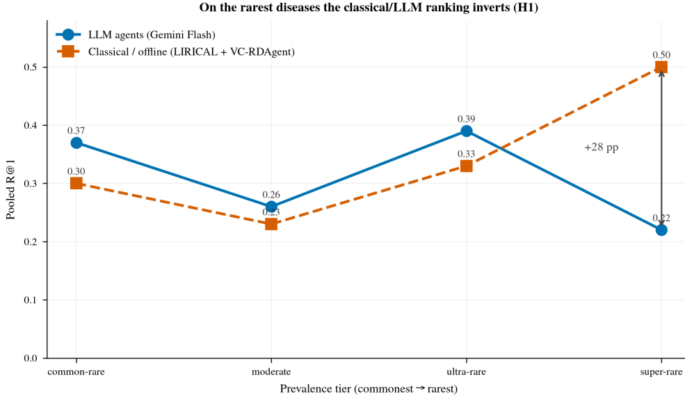
Figure 4: Prevalence crossover (H1) . Pooled R@1 by Orphanet prevalence tier. LLM agents decline toward the rarest tier while classical/offline baselines rise, inverting the ranking on super-rare disease (+28 pp for classical).
