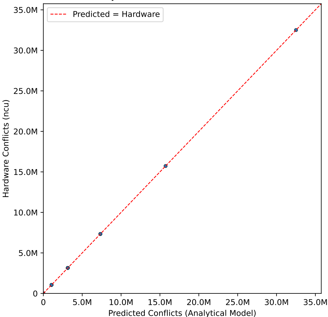
Analytical Model vs Hardware Verification
