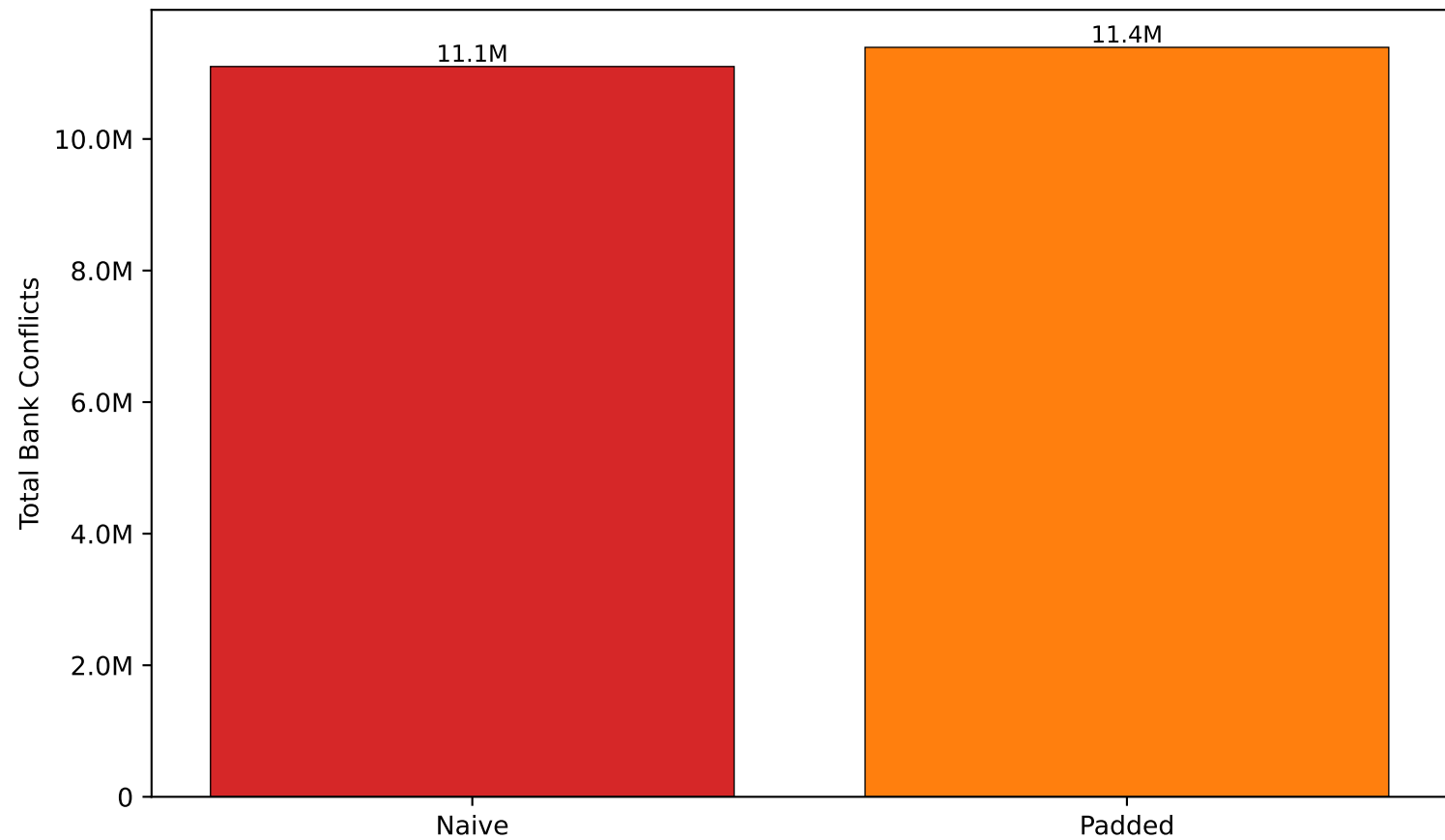
C++ BERT Runner (12 layers, \text{tile}_k=64 ): Naive vs Optimized Layouts (ncu)
