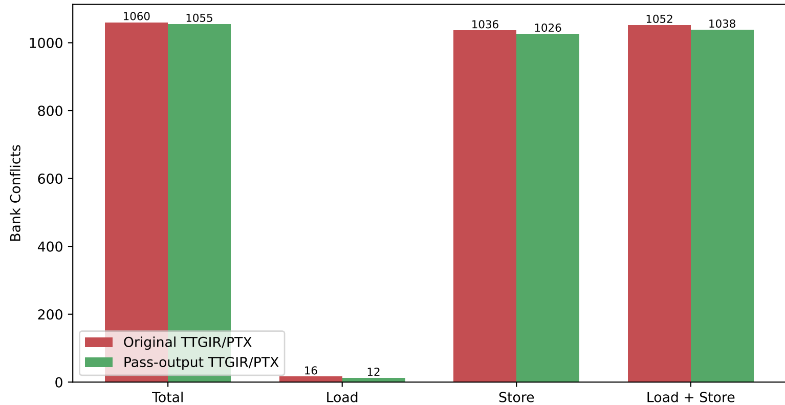
Pass-Driven GEMM: Input vs Output Bank Conflicts
