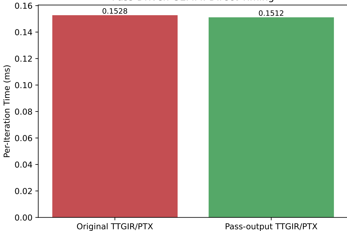
Pass-Driven GEMM: Direct Timing
