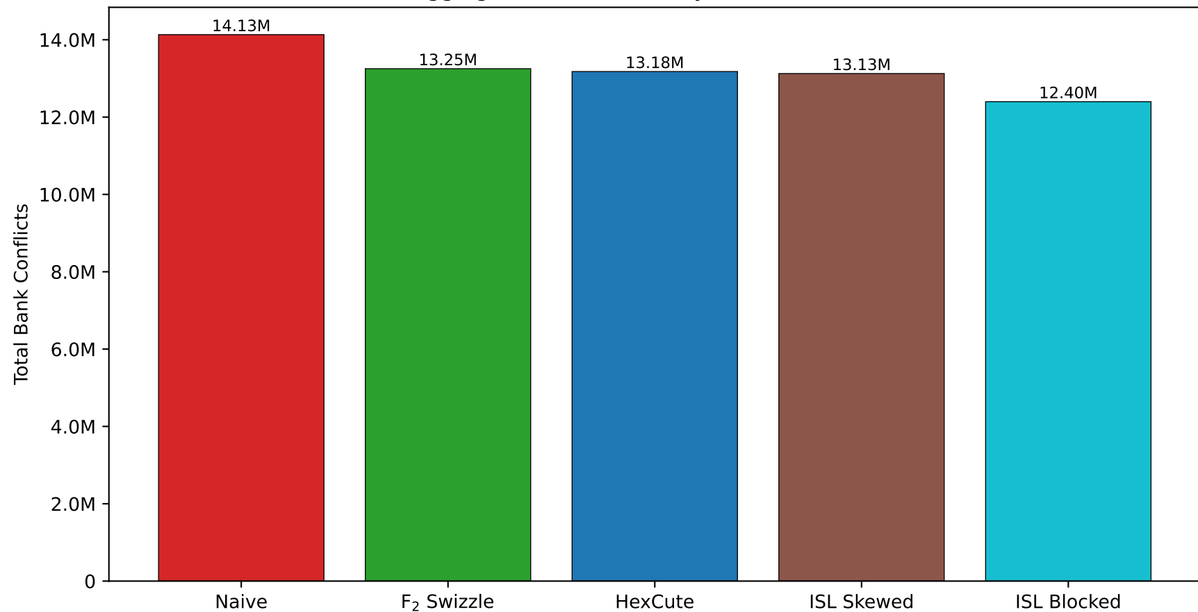
Real HuggingFace BERT: Five-Layout Total Bank Conflicts
