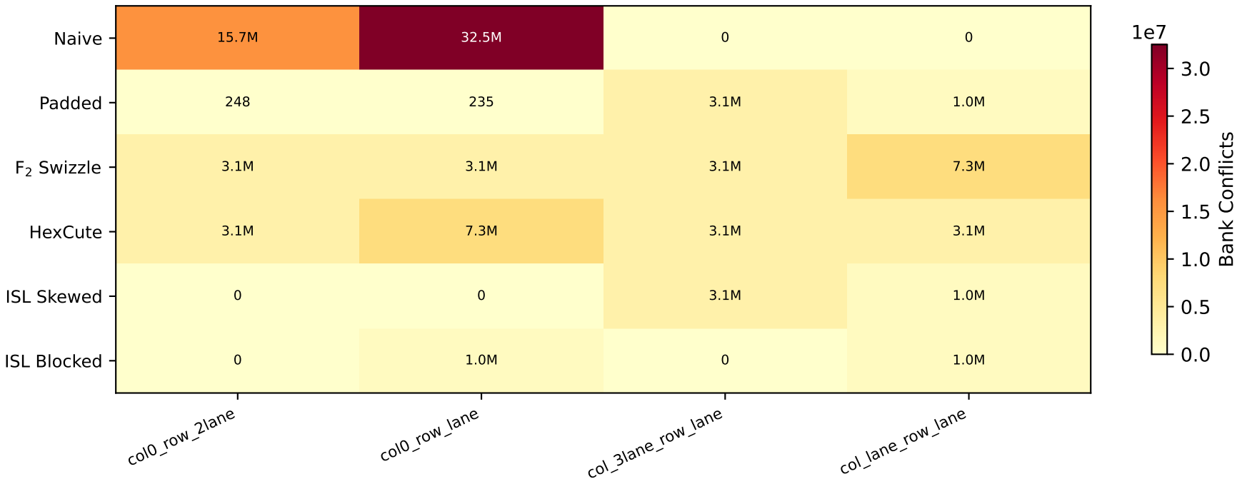
Stress-Kernel Conflicts by Layout and Pattern ( \text{tile}_k=64 , ncu)
