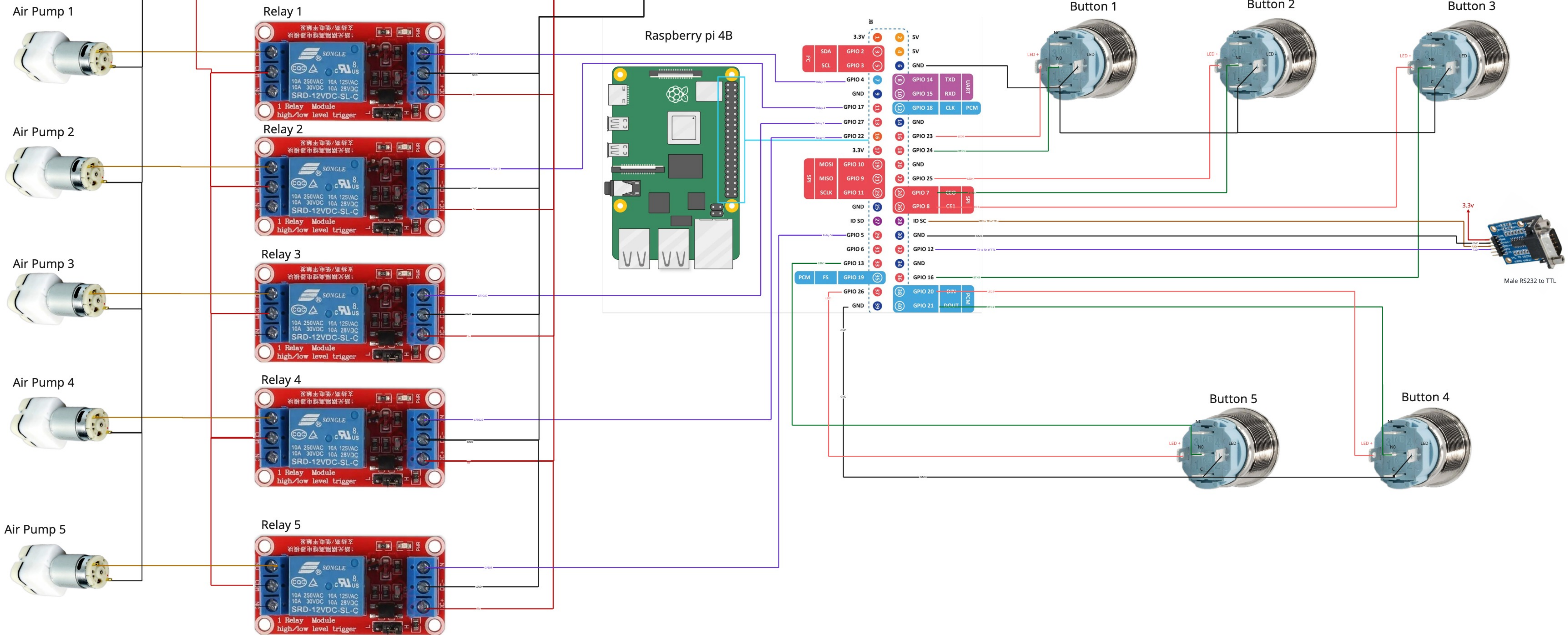
FIG : Perfume Dispenser Schematics Diagram v2
