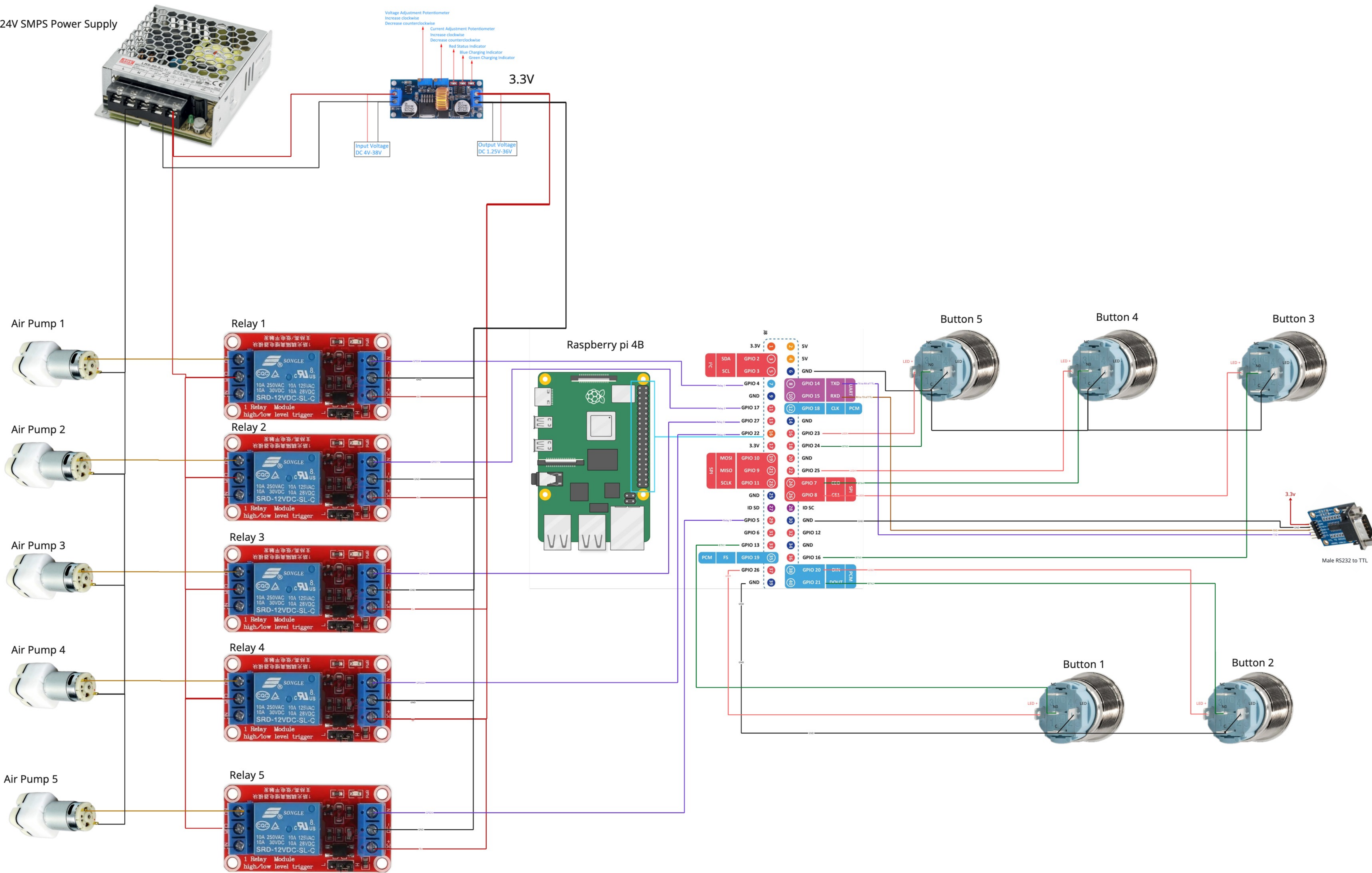
FIG : Perfume Dispenser Schematics Diagram v2.1
