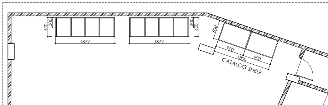
WALL DETAIL A AT GROUND FLOOR-PLAN
