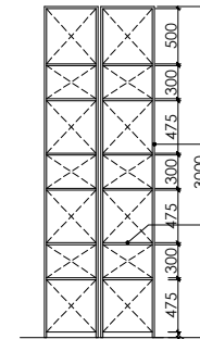
SHELF NEAR RECEPTION ELEVATION
