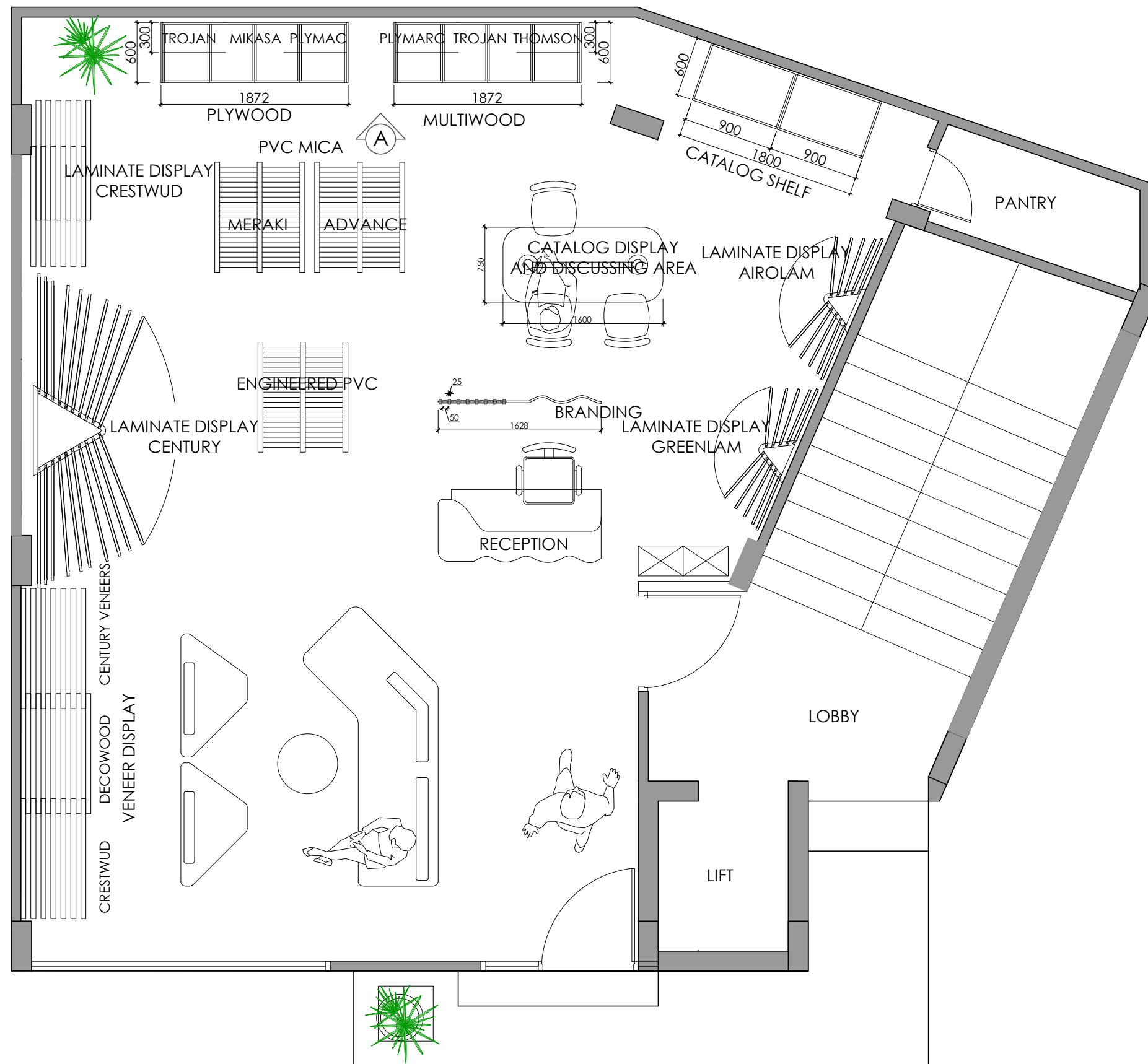
FURNITURE LAYOUT- GROUND FLOOR
