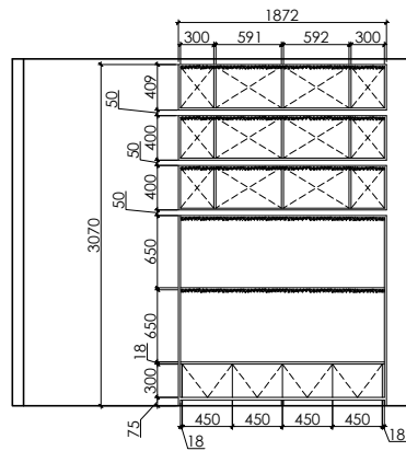
WALL DETAIL A ELEVATION
